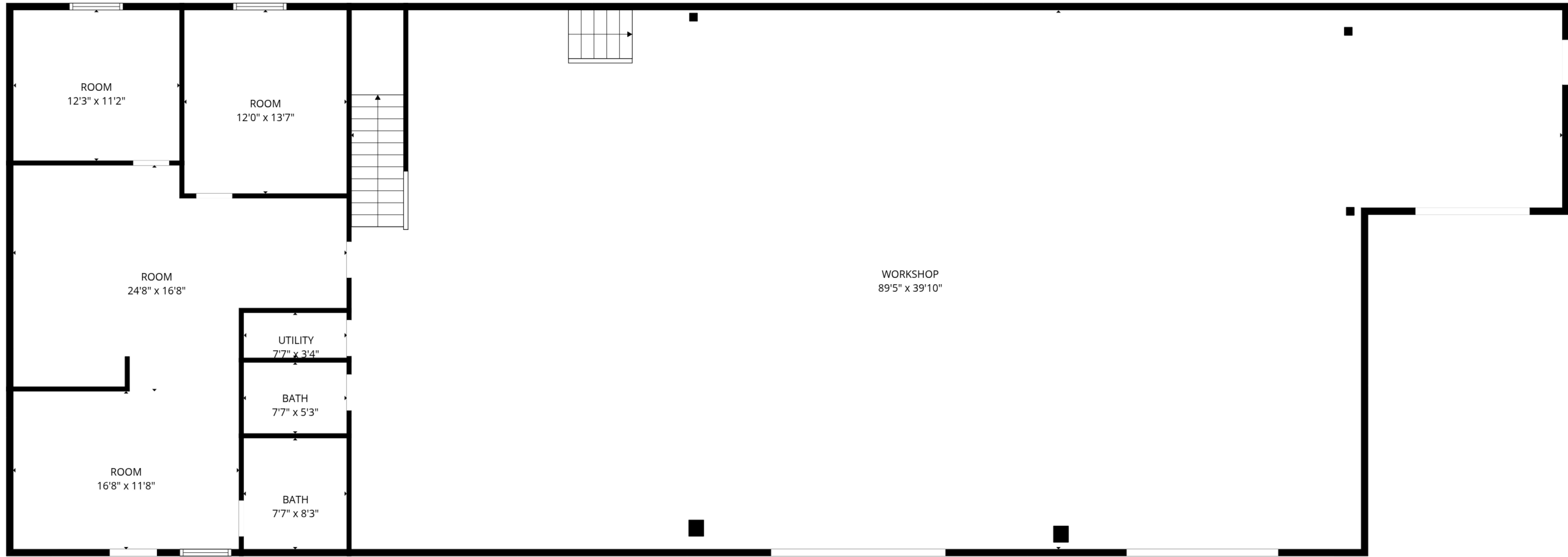
1st floor
