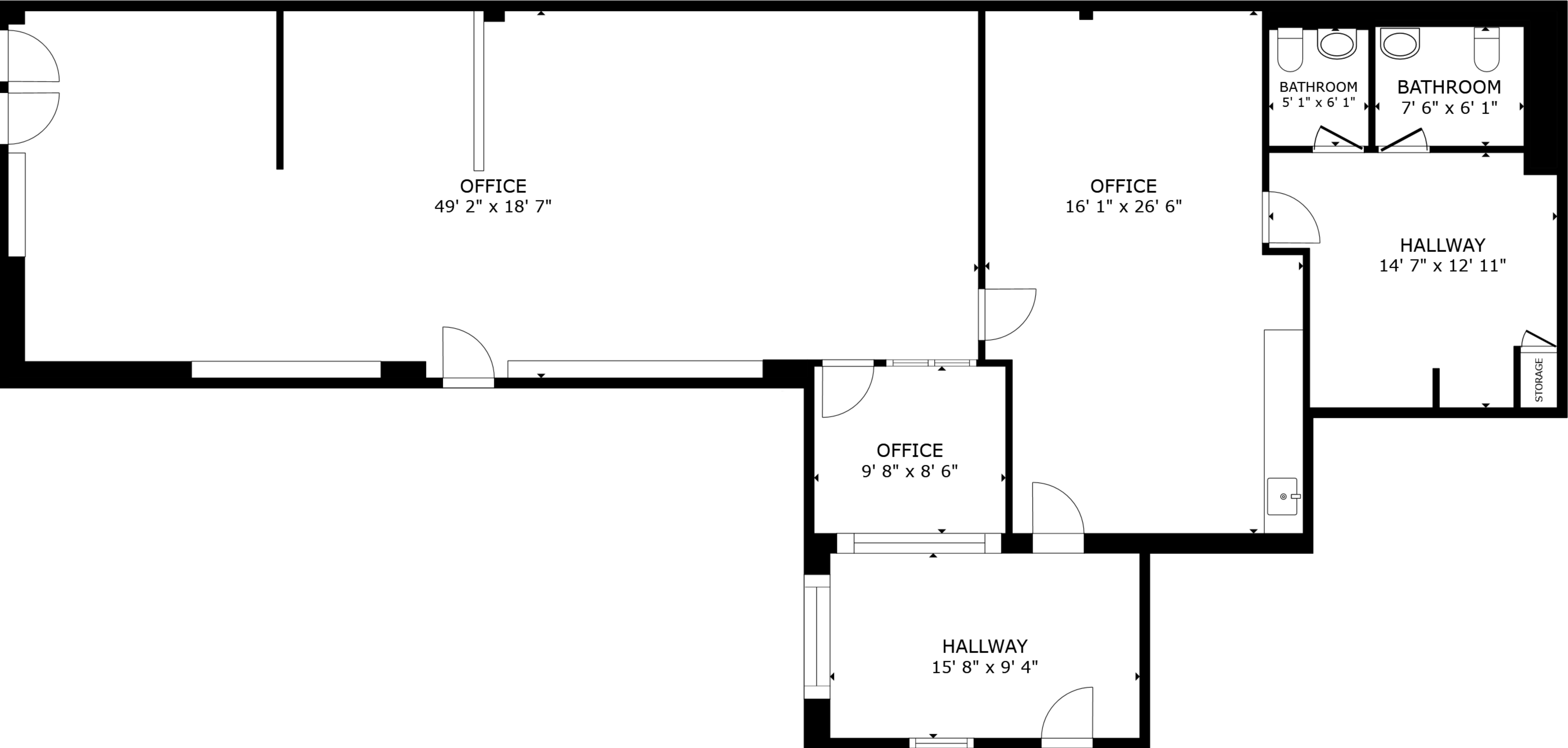
FLOOR PLAN
