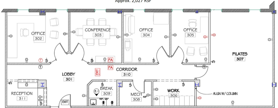
FLOOR PLAN 1/4" = 1'
