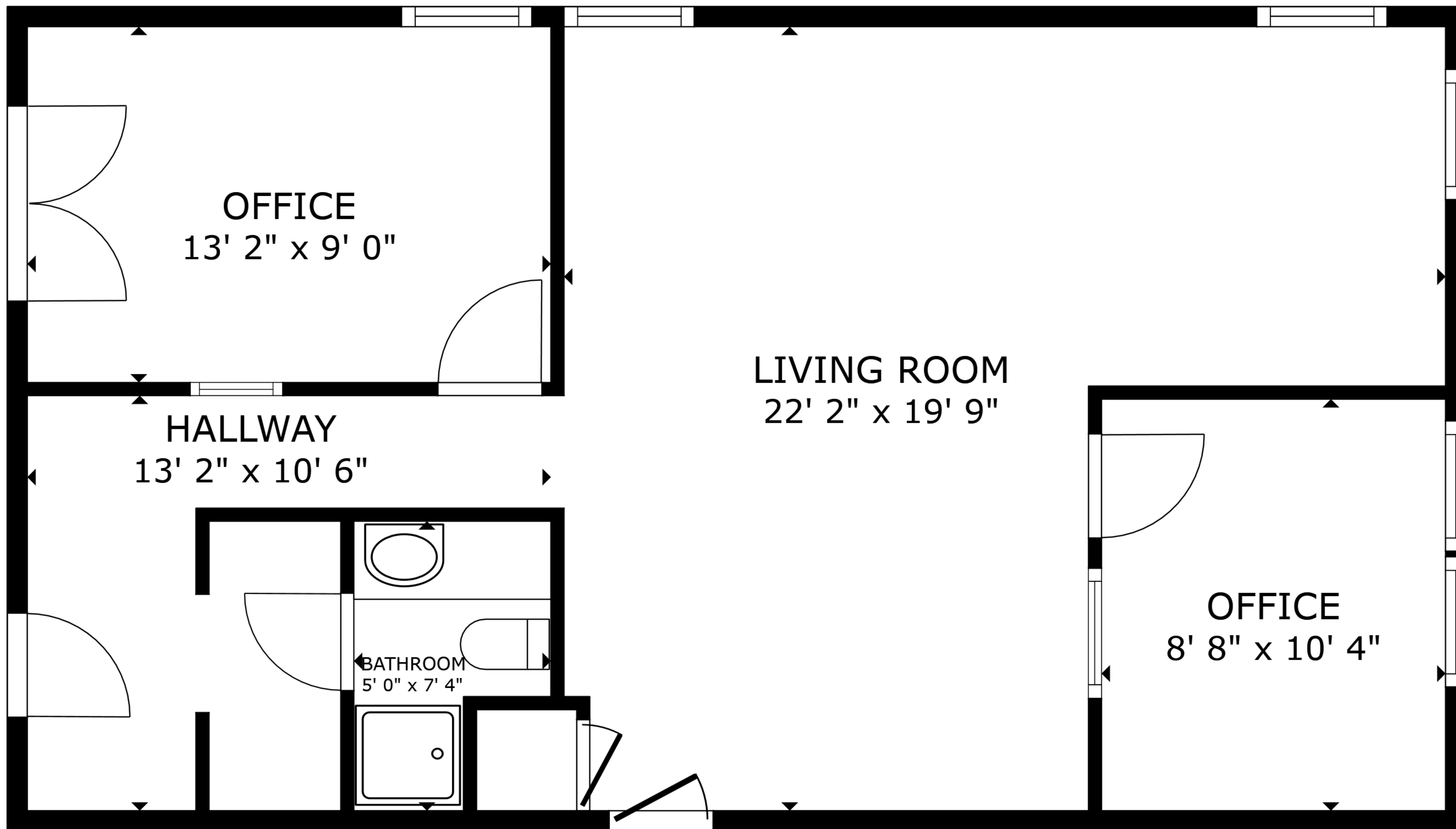
FLOOR PLAN
