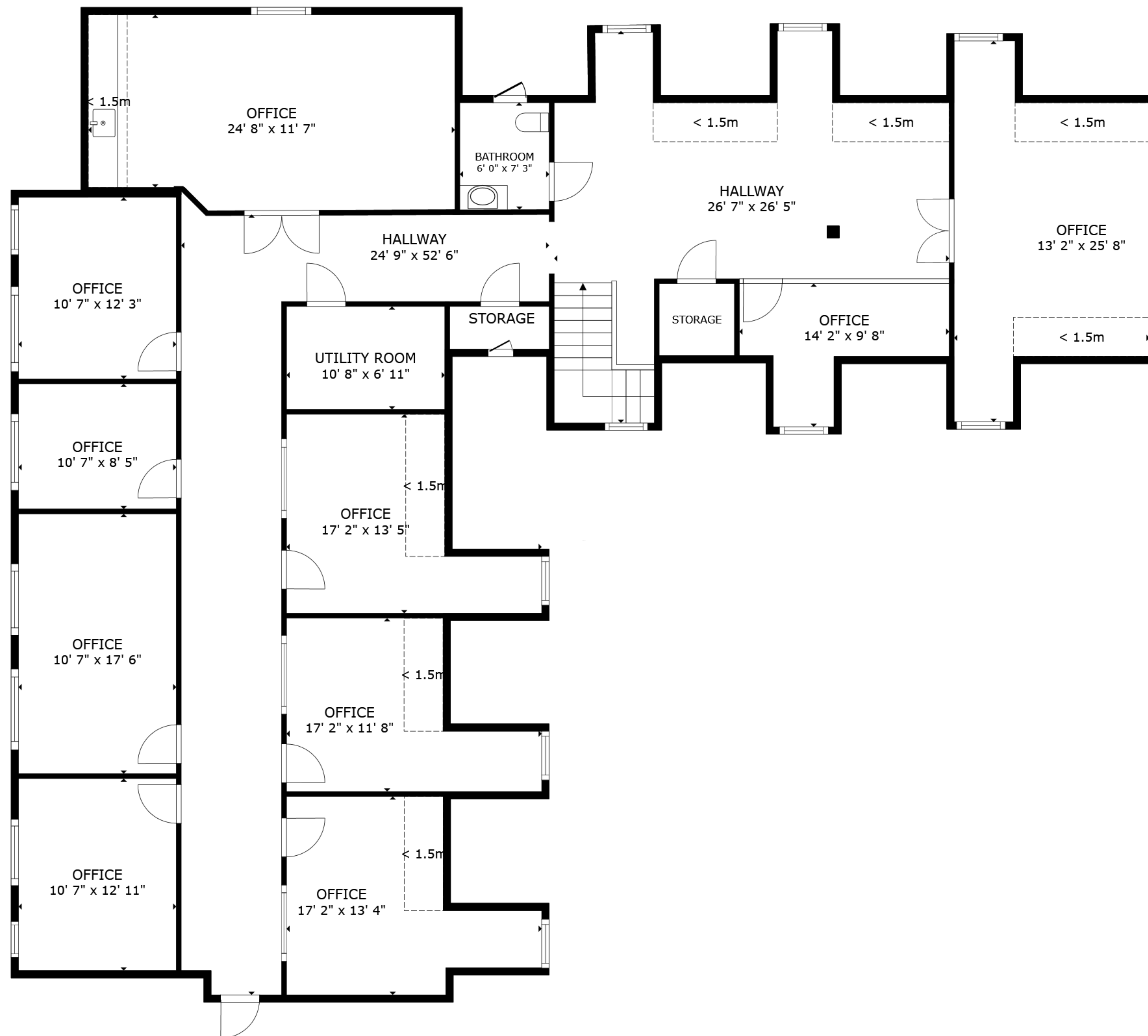
FLOOR PLAN
