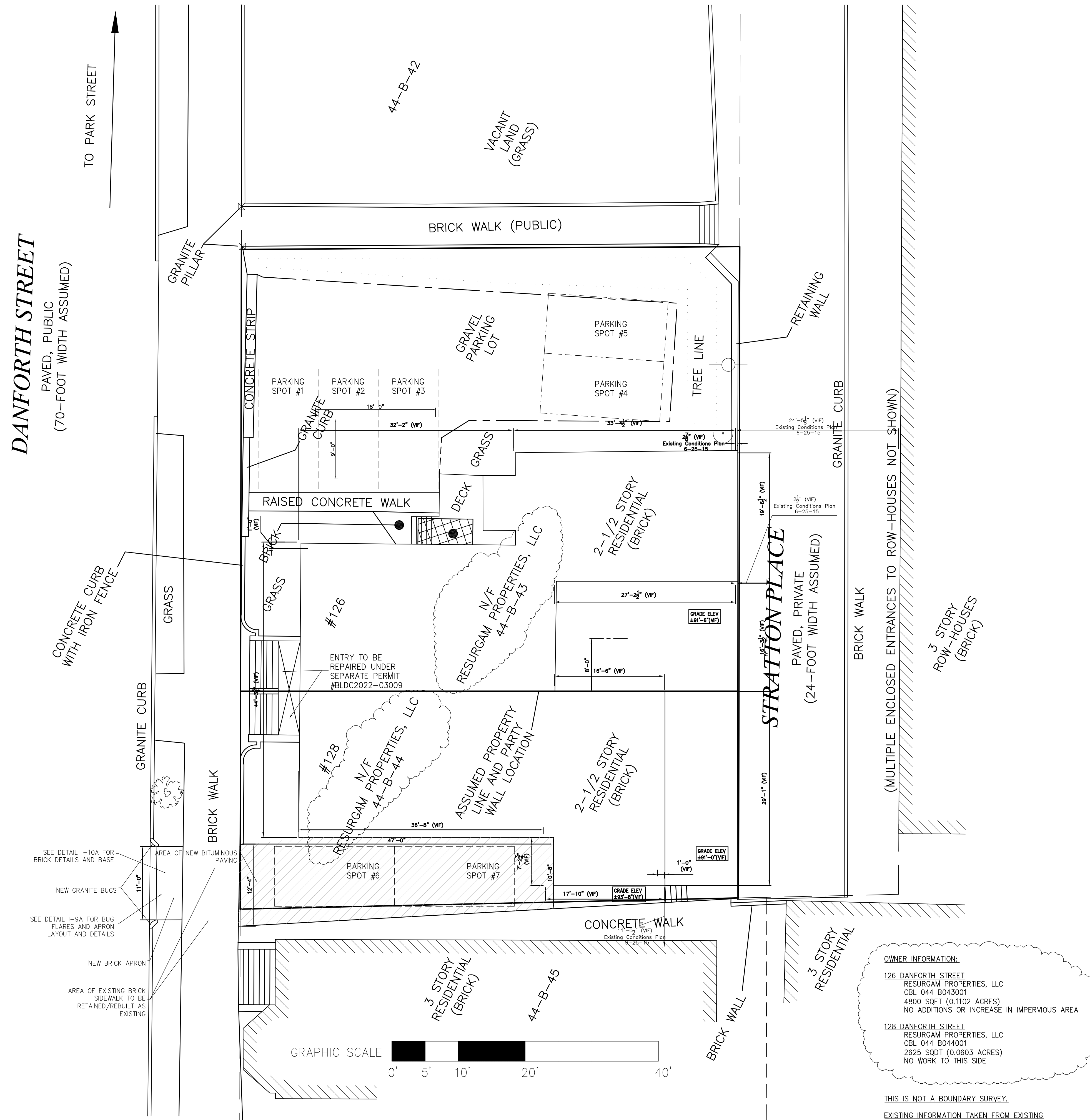
2 PLOT PLAN 1/8" = 1' - 0"
