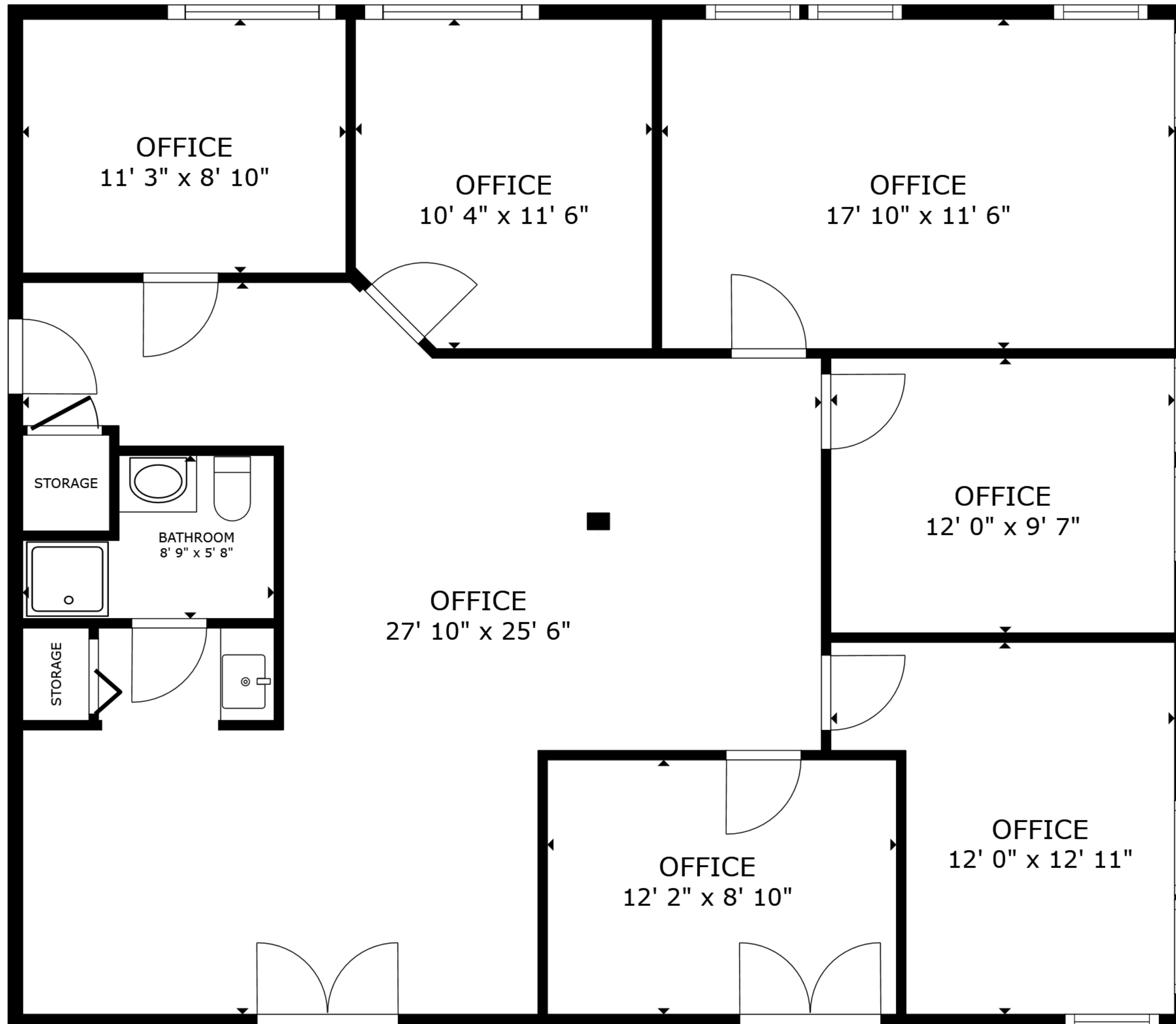
FLOOR PLAN
