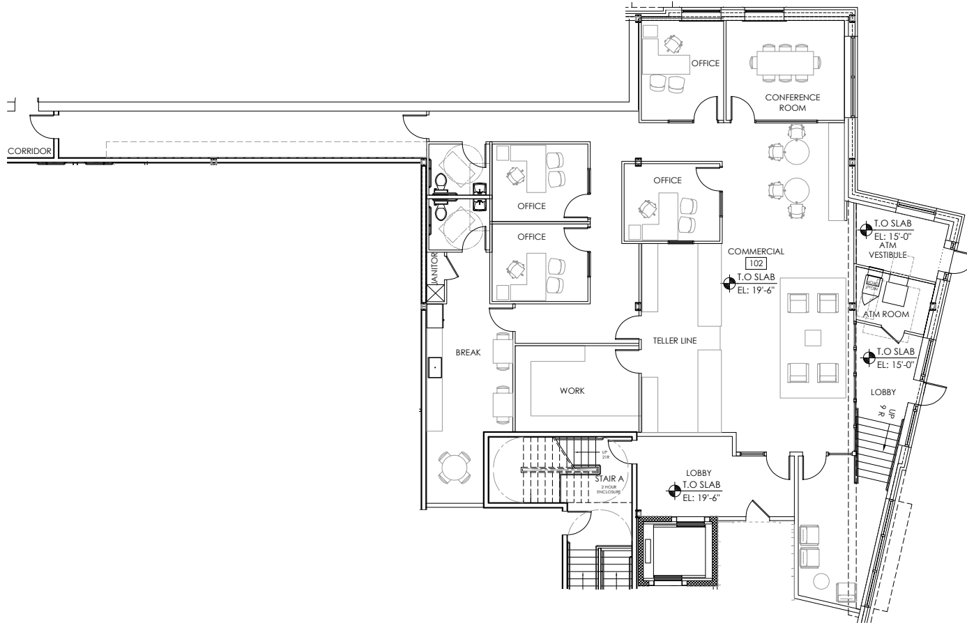
1 BANK FITUP PLAN 3/32" = 1'-0"
